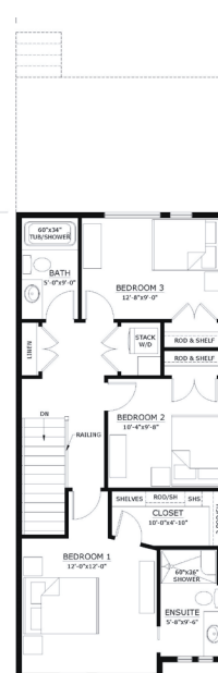
UPPER FLOOR
