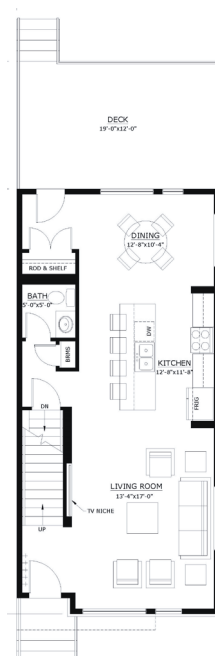
MAIN FLOOR
