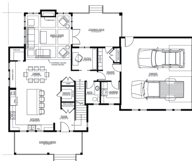
MAIN FLOOR
