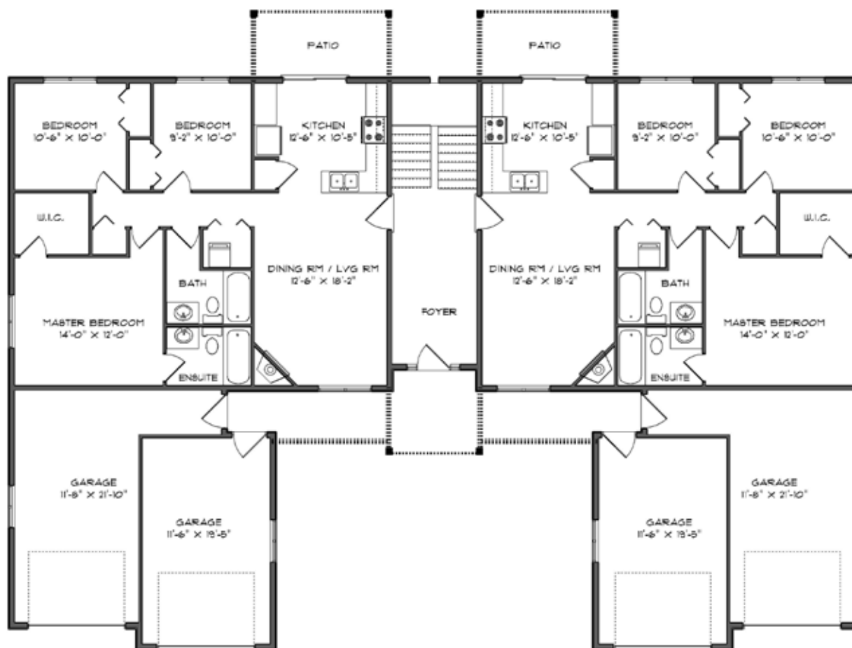
MAIN FLOOR
