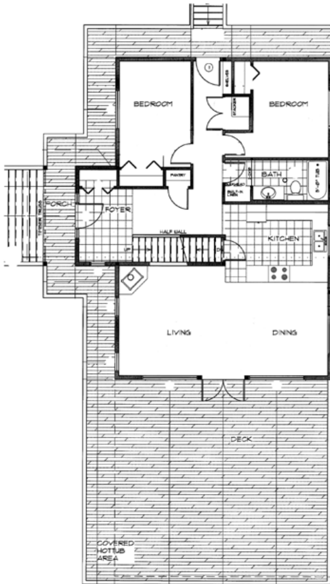
MAIN FLOOR
